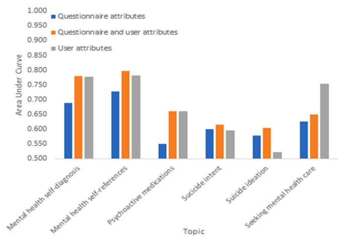
Fig. 3. Area Under Curve (AUC) for predicting respective outcomes. Independent attributes are the attributes of the screening tools, user attributes, or both.
